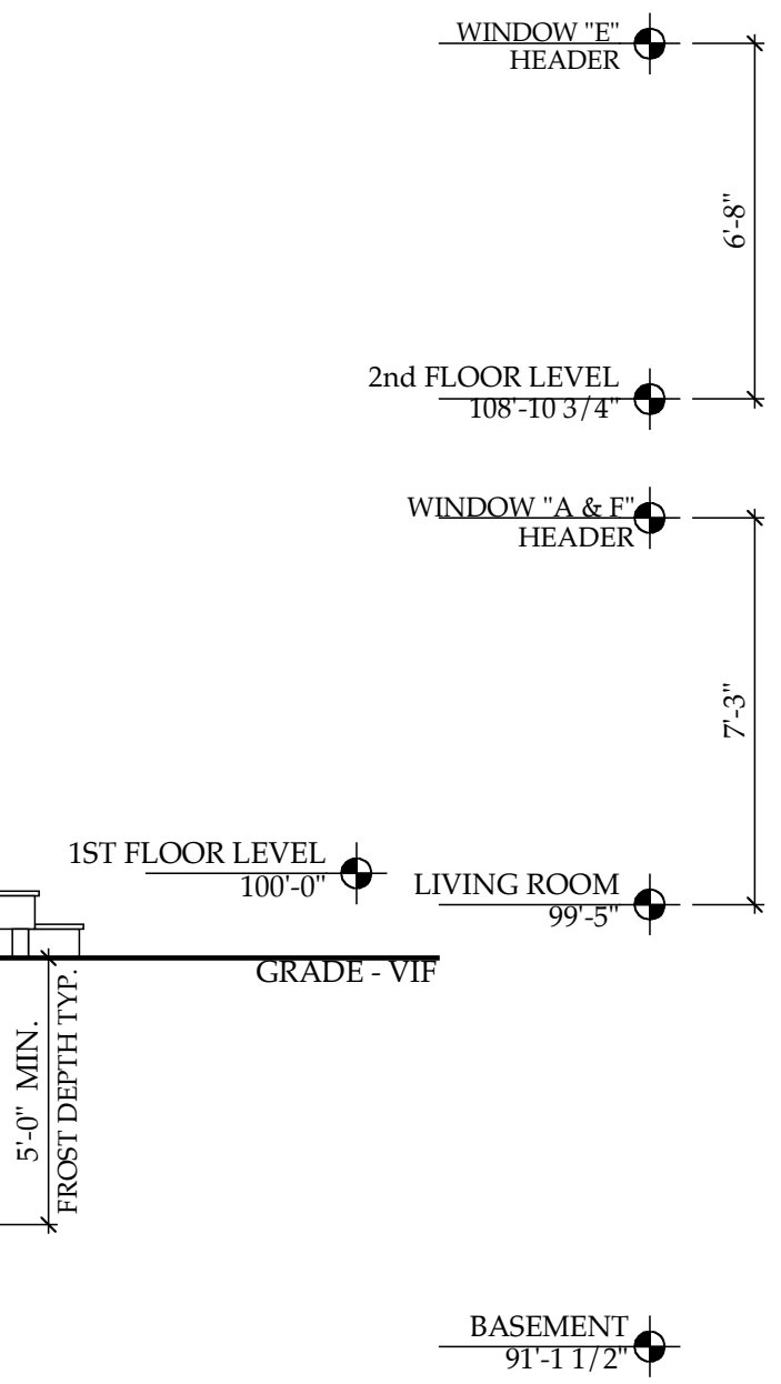
WEST ELEVATION
