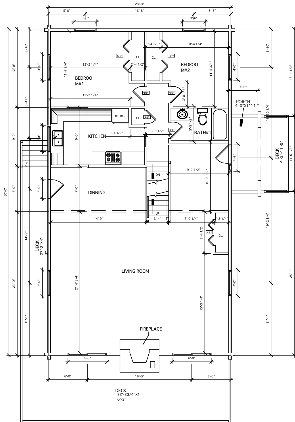
FRIST FLOOR PLAN
