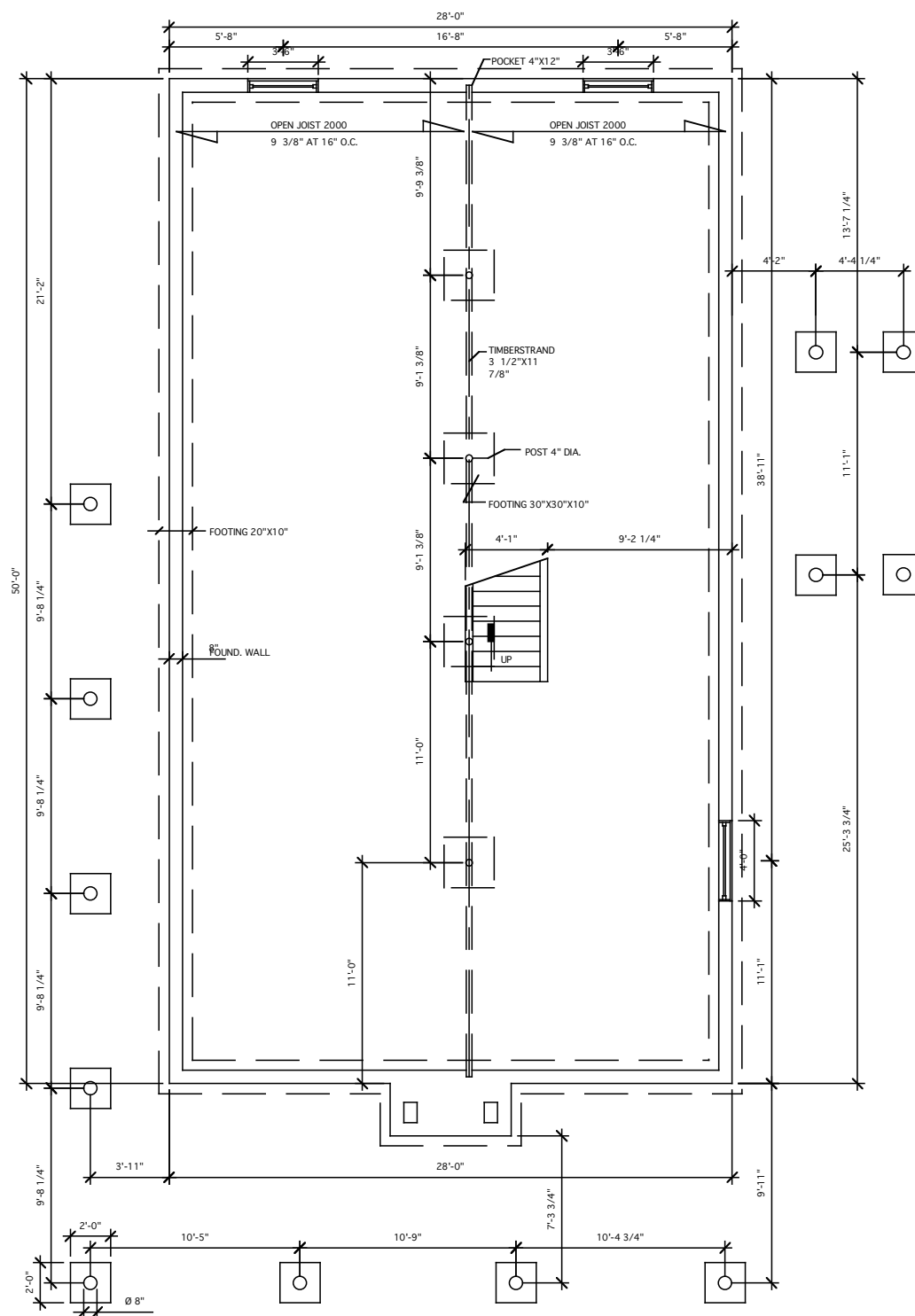
FOUNDATION PLAN
