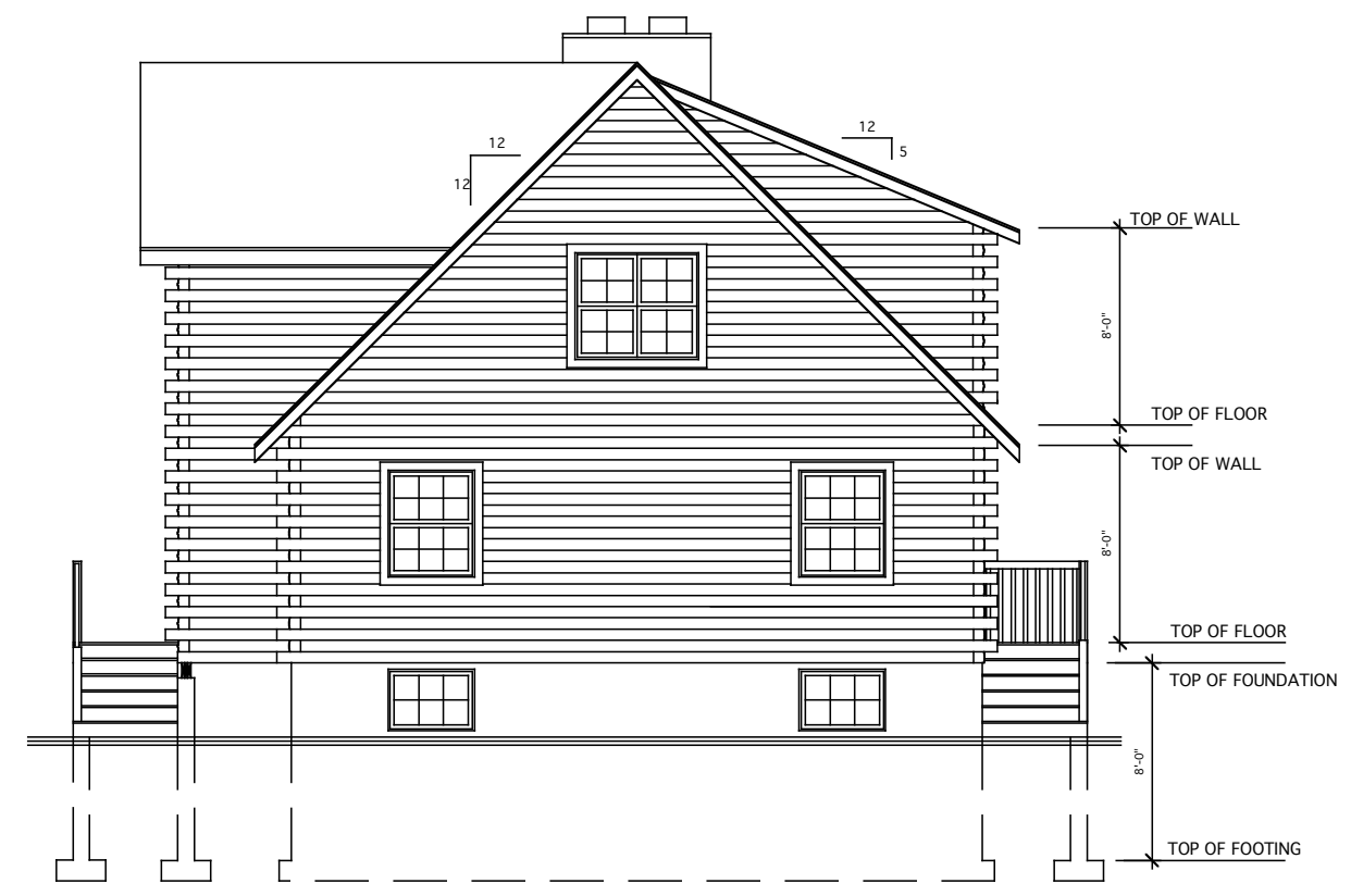
REAR ELEVATION
