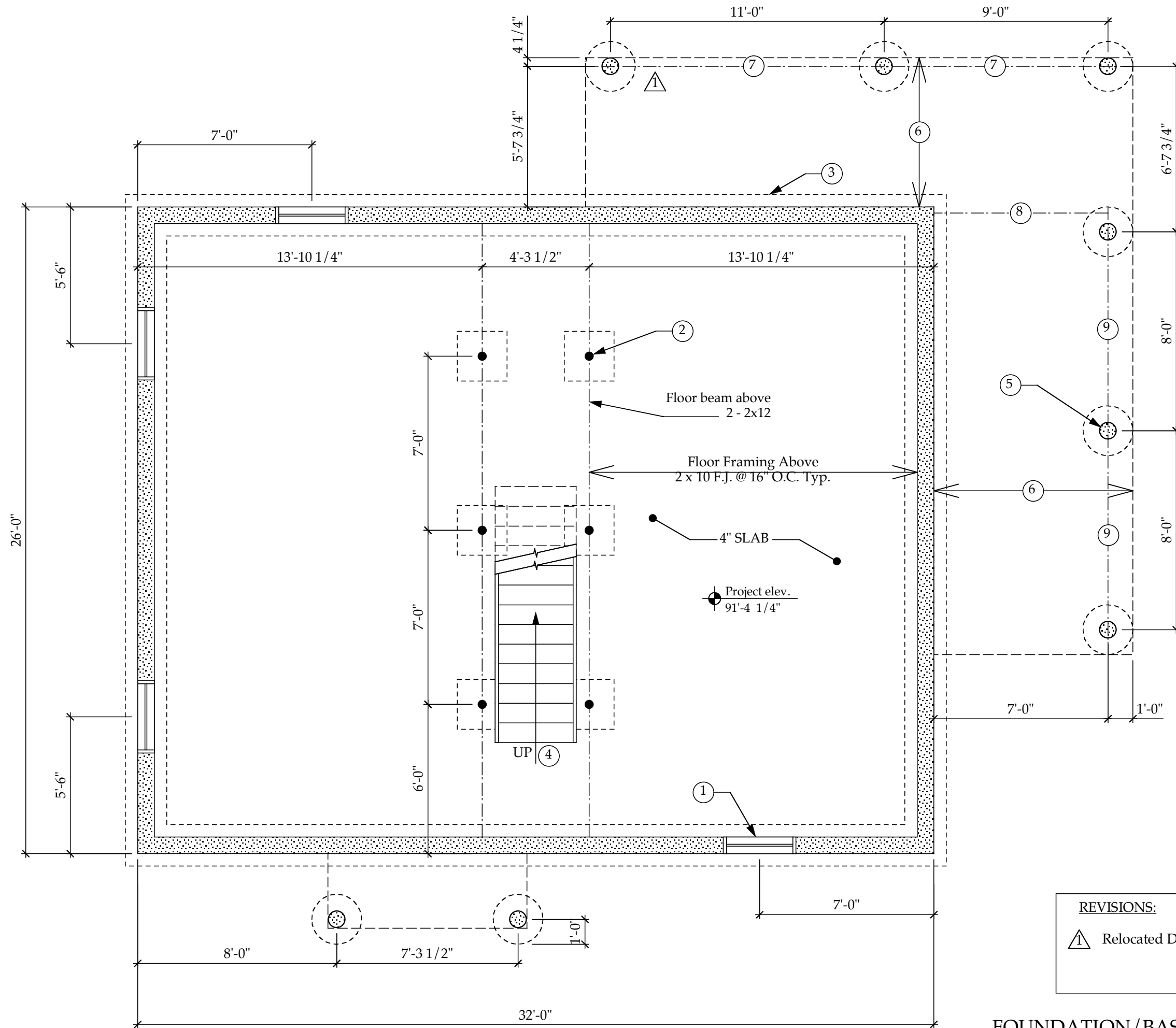
FOUNDATION/BASEMENT PLAN
